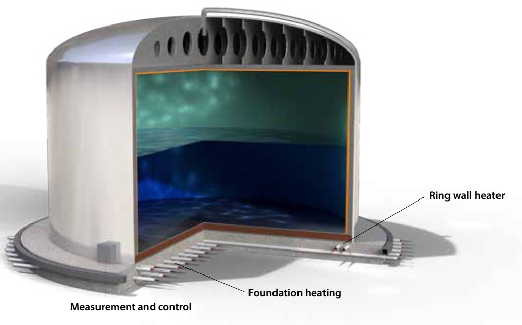
Schematic overview of a cryogenic tank base heating system
